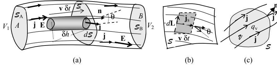
Figure 3.10. a) Lines of current and volume current density, b) surface current density, and c) conservation of electric charge
