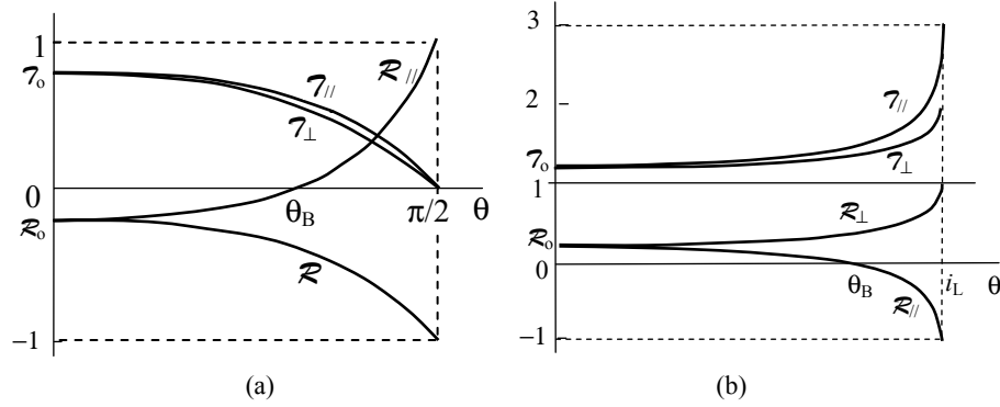
Figure 11.3. Variations of \mathcal{R}_\perp , \mathcal{R}_\parallel , \mathcal{T}_\perp and \mathcal{T}_\parallel versus \theta : a) if n_1 < n_2 (the graph corresponds to n_1 = 1 and n_2 = 1.5 ), and b) if n_2 < n_1 (the graph corresponds to n_1 = 1.5 and n_2 = 1 )
