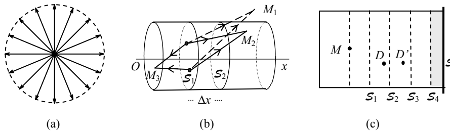
Figure 11.15. Diffusion of a wave: a) the superposition of randomly phased waves is completely destructive, b) propagation of a wave as interference of the diffused waves and the primary wave, and c) reflection as interference of diffused wavelets
