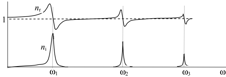
Figure 10.6. Typical variations of the real part of the index of refraction and its imaginary part
