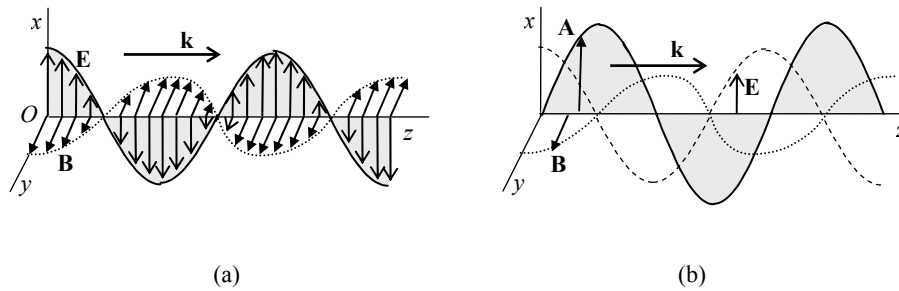
Figure 10.2. a) Plane electromagnetic wave that is polarized linearly in the direction Ox , propagating in the direction Oz if it is represented by the fields \mathbf{E} and \mathbf{B} . b) The same wave represented by the vector potential \mathbf{A} in the Coulomb gauge
