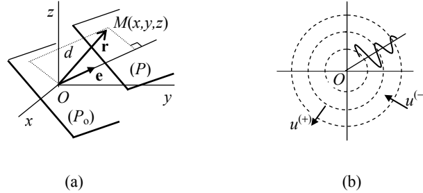
Figure 10.1. a) Three-dimensional plane wave and b) spherical wave
