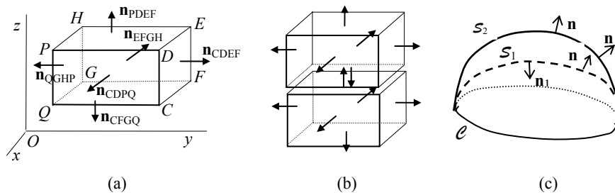
Figure A.3 a) Gauss-Ostrogradsky's theorem for an infinitesimal parallelepiped; b) flux through two adjacent parallelepipeds; c) conservation of the flux through the surfaces bounded by the same closed path \mathcal{C} if \nabla \cdot \mathbf{B} = 0
