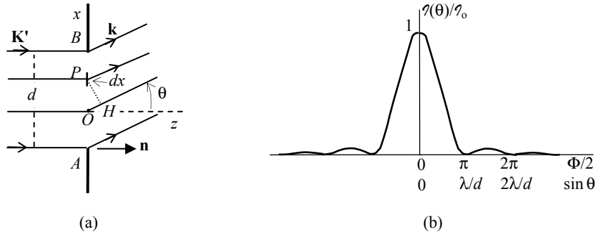
Figure 11.8. a) Diffraction by a slit AB of width d in the case of a normal incident wave, and b) variation of the intensity as a function of \Phi/2 or \sin \theta
