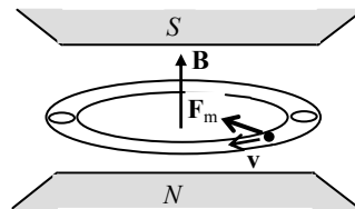
Figure 8.10. The betatron
