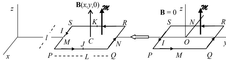
Figure 6.14. Evaluation of the interaction energy of an electric circuit in a field \mathbf{B}
