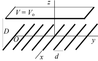
Figure 5.4. A grid parallel to a conducting plate
