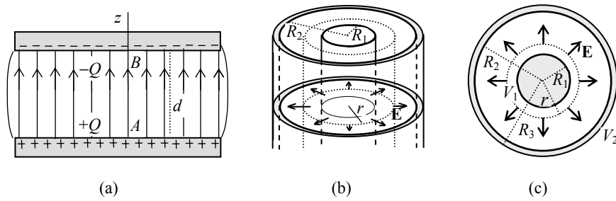
Figure 3.5. a) Parallel plate capacitor, b) cylindrical capacitor, and c) spherical capacitor
