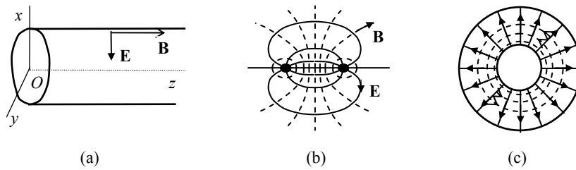
Figure 12.3. a) Electromagnetic waveguide in the form of a hollow conductor, b) waveguide formed by two parallel conducting wires, and c) coaxial cable. The lines of \mathbf{E} are drawn as solid lines and those of \mathbf{B} are drawn as dashed lines
