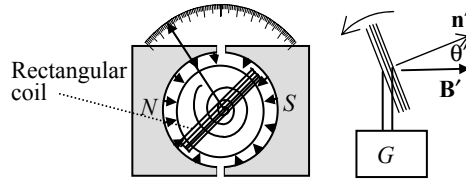
Figure 8.8. Galvanometer and measurement of B
