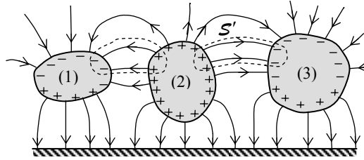
Figure 3.7. Conductors in mutual influence
