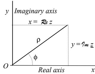
Figure A.1. Argand diagram for complex numbers
