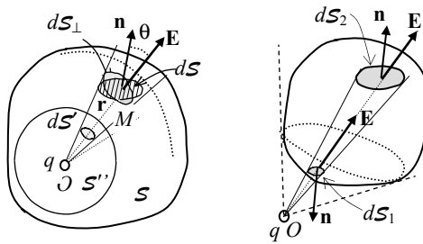
Figure 2.3. Gauss's law
