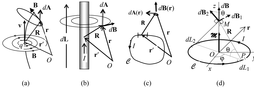
Figure 6.4. Magnetic field and vector potential a) of a charged particle of velocity \mathbf{v} , b) of a circuit element d\mathbf{L} (Biot-Savart's law), c) of a finite thin circuit, and d) of a circular loop
