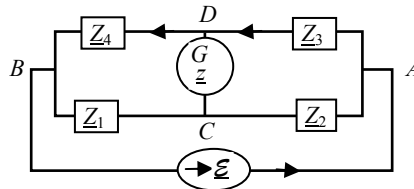
Figure 3.17. Wheatstone bridge
