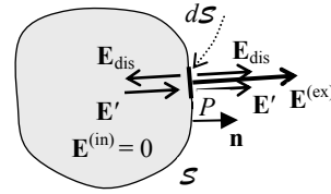
Figure 3.9. Electrostatic pressure
