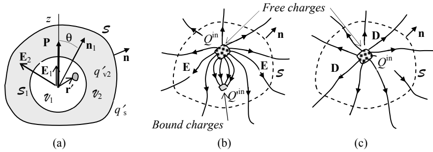
Figure 4.4. a) Evaluation of \mathbf{E} in a dielectric. b) Gauss's law \Phi_E = (Q^{(in)} + Q'^{(in)})/\epsilon_0 uses both free charges Q^{(in)} and bound charges Q'^{(in)} inside \mathcal{S} . c) It may be written also as \Phi_D = Q^{(in)}/\epsilon_0
