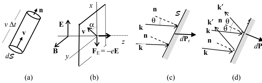
Figure 10.5. a) Interpretation of the relation \mathbf{S} = vU_{\text{EM}}\mathbf{e} . Radiation pressure of a wave that is b) incident normally on a totally absorbing plate, c) incident obliquely on a totally absorbing body, and d) incident obliquely on a totally reflecting body
