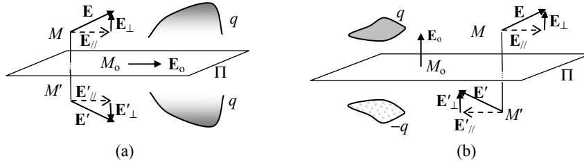
Figure 2.5. a) Symmetry with respect to a plane \Pi , and b) antisymmetry with respect to \Pi
