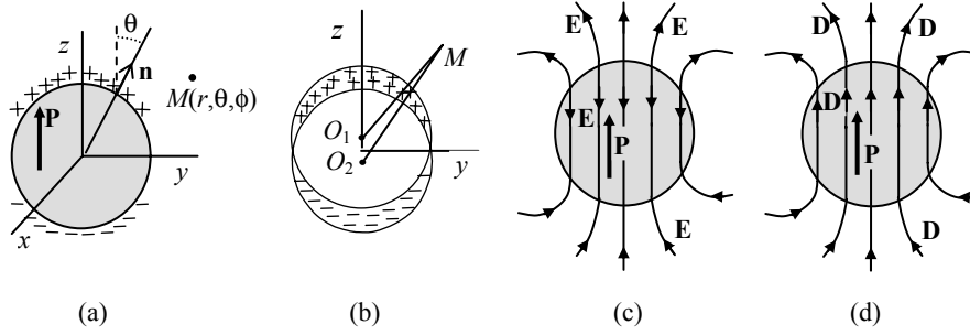
Figure 4.7. Polarized ball: a) the surface polarization charge density, b) its equivalence to two balls of opposite charges, c) lines of the field \mathbf{E} , and d) lines of the field \mathbf{D}
