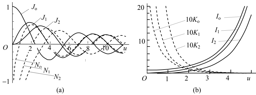
Figure 5.6. Bessel functions
