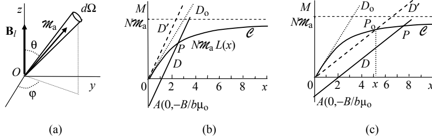
Figure 7.10. a) Orientation of the magnetic moment, b) magnetization if T > T_W , and c) magnetization if T < T_W
