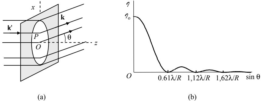
Figure 11.9. a) Diffraction by a circular aperture, and b) variation of the intensity as a function of \sin \theta , where \theta is the angle of observation
