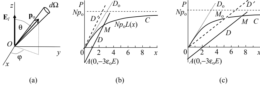
Figure 4.10. Polarization of a polar substance: a) orientation of the dipole moment \mathbf{p}_o , b) polarization for T > T_c , and c) polarization for T < T_c
